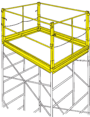
Panel Guard System in application.
