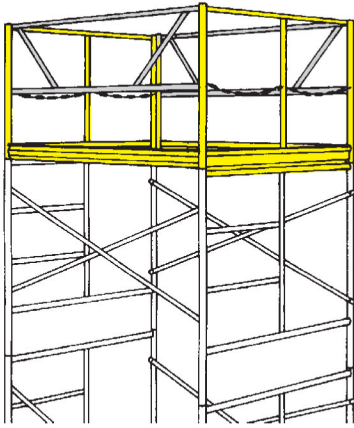
Easi-Guard System in application.
