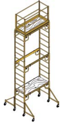
0127-006-3 2 Single Units, 1-65" Additional Height Unit w/Guard Rail & 24" Wide Outriggers
