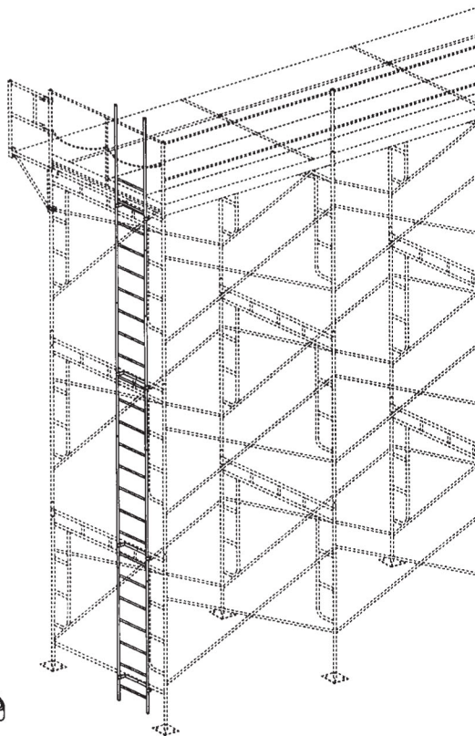
6' Ladder Section 0004-0375
