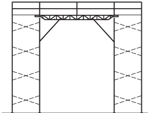
Typical Putlog Application Shown.
