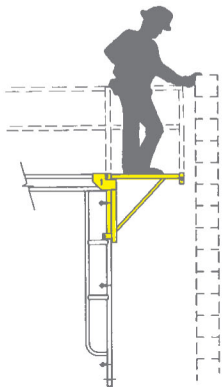
Side Bracket Shown in Application.
